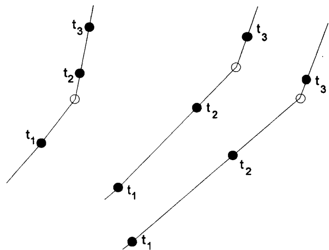
Figure 2. Points on three rays forming a ray tube in the place where the rays cross an interface. Filled circles represent the points at three traveltime levels t_1 , t_2 and t_3 (' time points '). Open circles are the points of intersection of the rays with the structural interface (' interaction points ').
