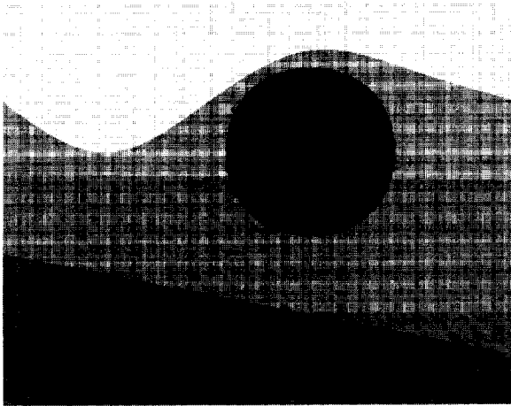
Figure 9. P -wave velocity cross-section through the middle of model '98'. The P -wave velocity is lowest at the top water layer and highest within the spherical body.
