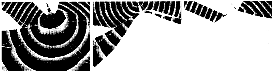
Figure 13. The single-valued traveltimes maps sorted according to the ray histories from Fig. 12, merged into the three sections. Some computed traveltimes were omitted.
