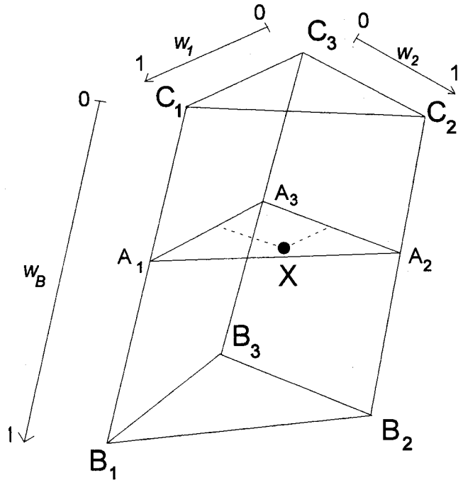
Figure 4. A ray cell is defined by six points B_1, B_2, B_3, C_1, C_2, C_3 , situated on three rays. Point X is examined to find out whether it is located within the ray cell. Its position may be expressed using the local coordinate system parametrized by parameters w_1, w_2, w_B . If all of the quantities w_1, w_2, w_B, 1 - w_1 - w_2 are in the range \langle 0, 1 \rangle , point X lies within the ray cell.
